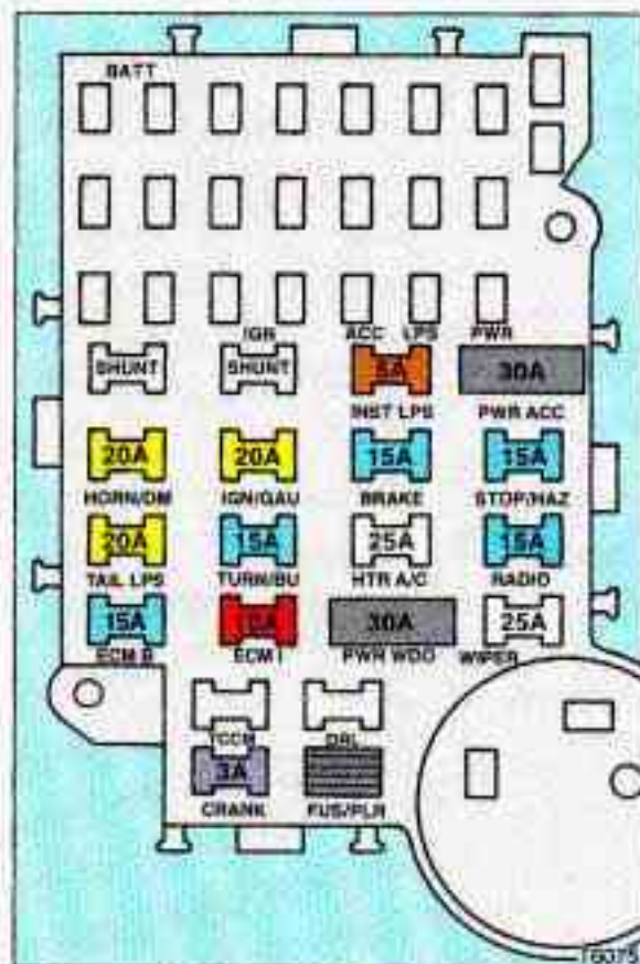
Fuse Usage
