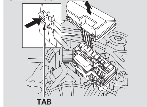
UNDER-HOOD
