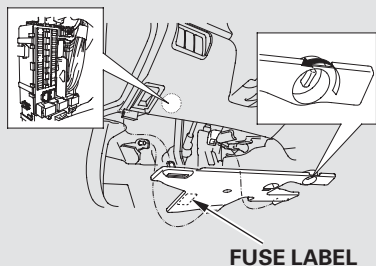
FUSE LABEL
